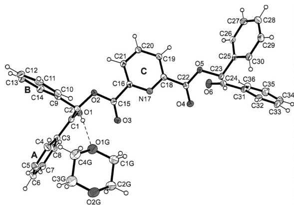
Fig. 1. Perspective view of 2a · 1,4-dioxane (1 : 1), including numbering scheme of atoms and ring specification. Displacement ellipsoids are at the 50 % probability level.
