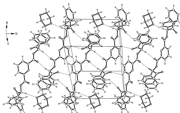
Fig. 2. Packing diagram of 2a · 1,4-dioxane (1 : 1). Oxygen atoms are displayed as dotted, nitrogen atoms as hatched and carbon atoms of the guest molecules as grey circles. Broken lines represent hydrogen bond interactions.
