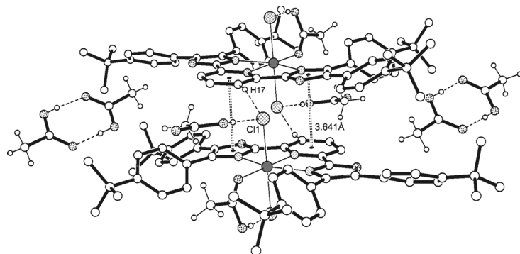
Fig. 6. Representation of the dimeric unit of the Ni(II) complex of 1c . Hydrogen bond interactions are displayed as broken lines; broken double lines represent arene face-to-face interactions. Non-relevant hydrogen atoms of the bisoxazole molecules are omitted for clarity.
