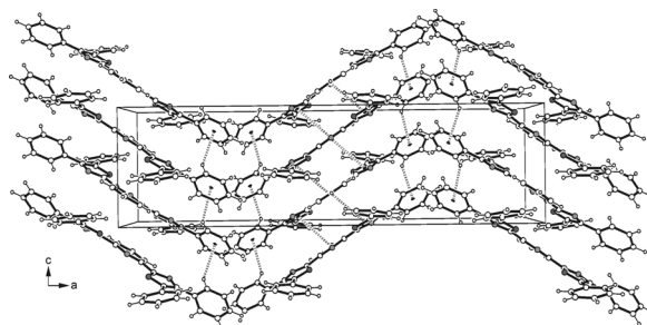
Fig. 4. Packing diagram of 1a viewed along the crystallographic b axis. Broken double lines represent aromatic face-to-face interactions.
