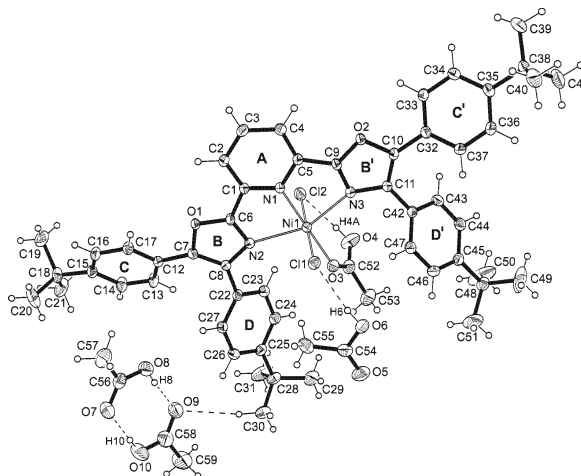
Fig. 5. Perspective view of [\text{Ni}(\text{1c})\text{Cl}_2(\text{HOAc})] \cdot 3\text{HOAc} , including numbering scheme of atoms and ring specification. Displacement ellipsoids are at the 50 % probability level. Thus lines represent coordinative bonds, broken lines hydrogen bond-type interactions.
