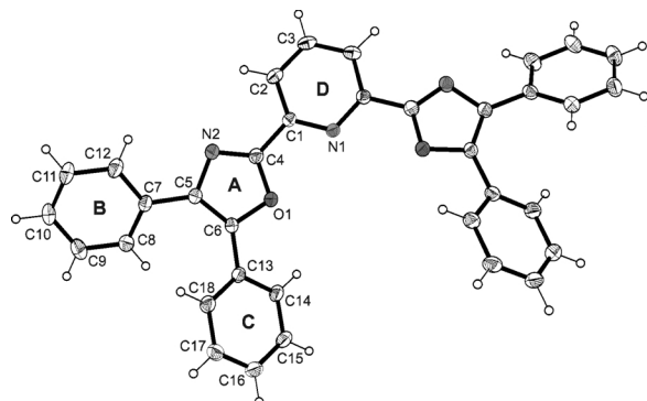
Fig. 3. Perspective view of 1a , including numbering scheme of atoms and ring specification. Displacement ellipsoids are at the 50 % probability level.
